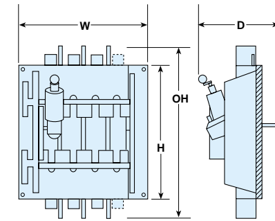
FIGURE 4: REAR CONNECTED
