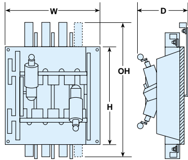
FIGURE 3: FRONT CONNECTED
