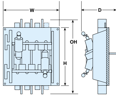
FIGURE 4: REAR CONNECTED
